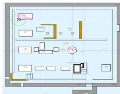
2. FLAIR-FLUKA geometria
